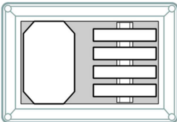
SMB-ADAPTOR with 1 CHQ-ADAPTOR (+ PCB) a DIN Rail and 4 CHQ-DIN Modules
